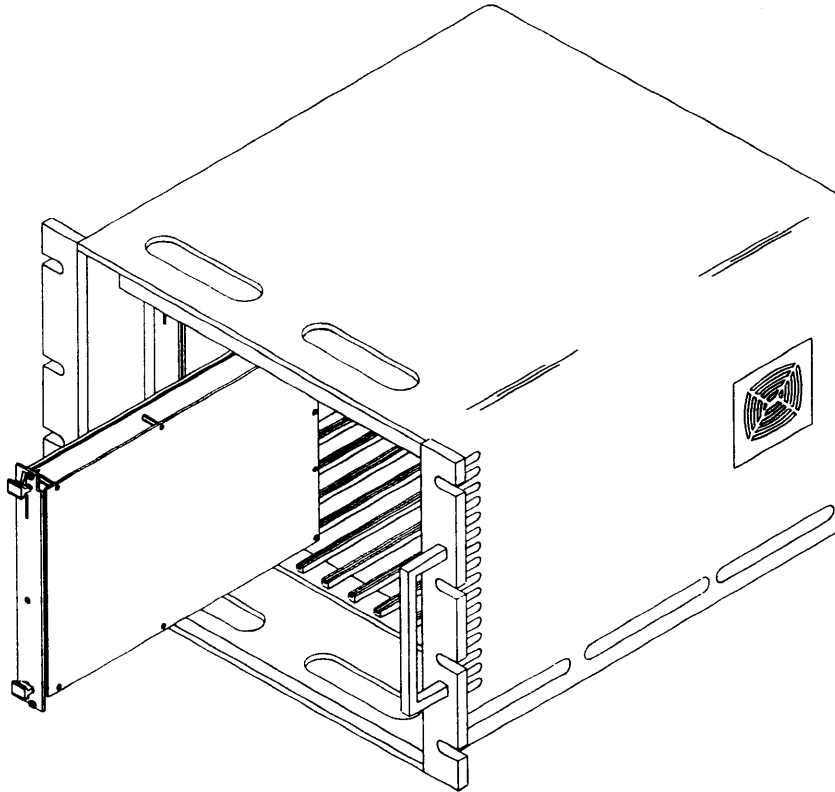
Figure 4: Module Installation
